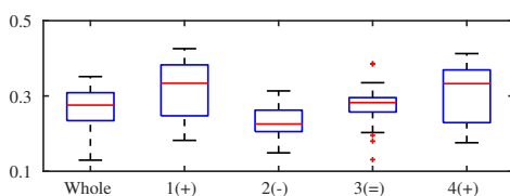
Fig. 4: The semantic similarity results for case 2.
